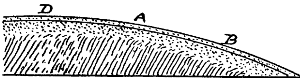
Figure 1 - Diagrammatic section of a hilltop indicating the zone of creep, and the position of the surface at two epochs.
